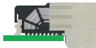
AirMax VS® Standard Profile SBB
