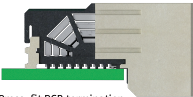
Press-fit PCB termination
