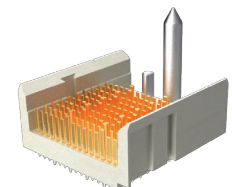
Vertical Receptacle (Right Guide)
