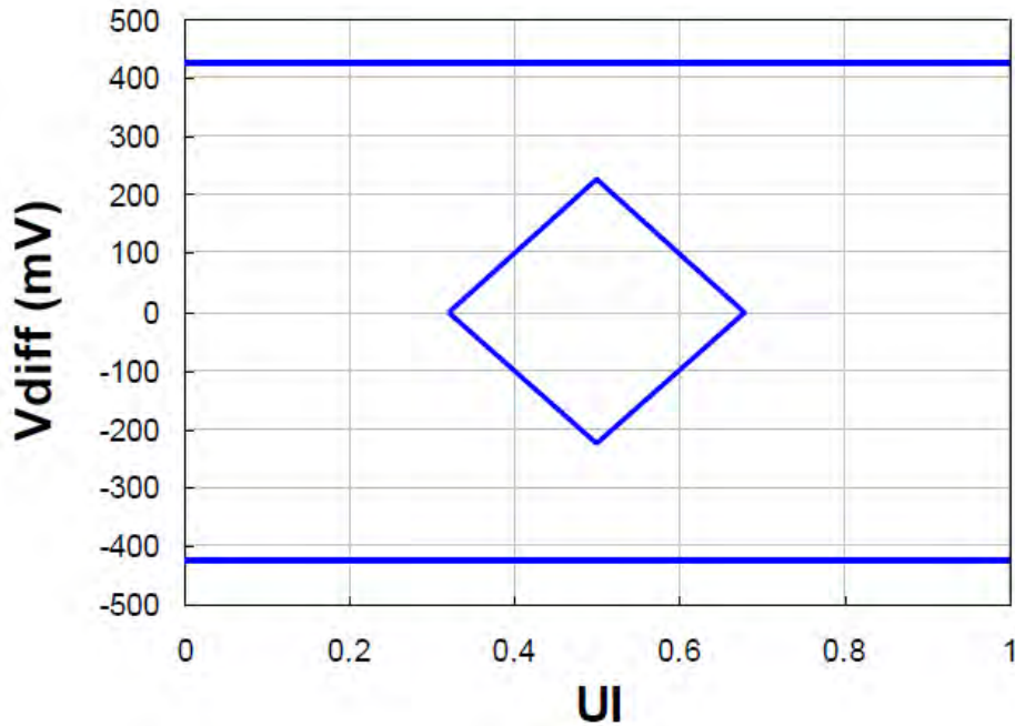
Figure 2 – Receiver Output Differential Signal Mask
