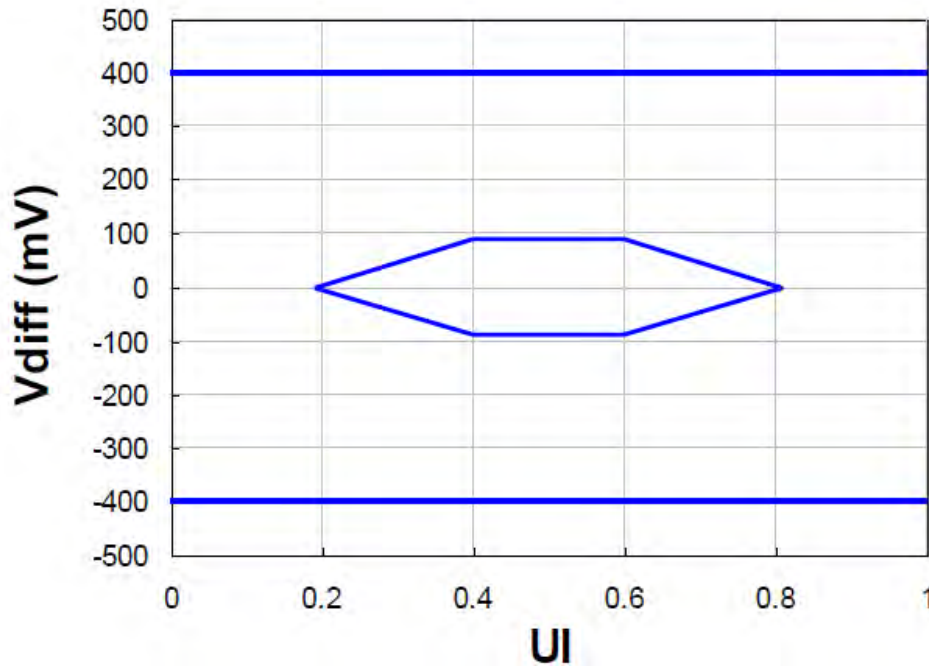
Figure 1 – Transmitter Input Differential Signal Mask
