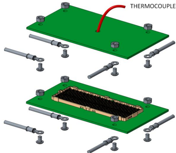
FIGURE 2 Maximum Current Set-up
