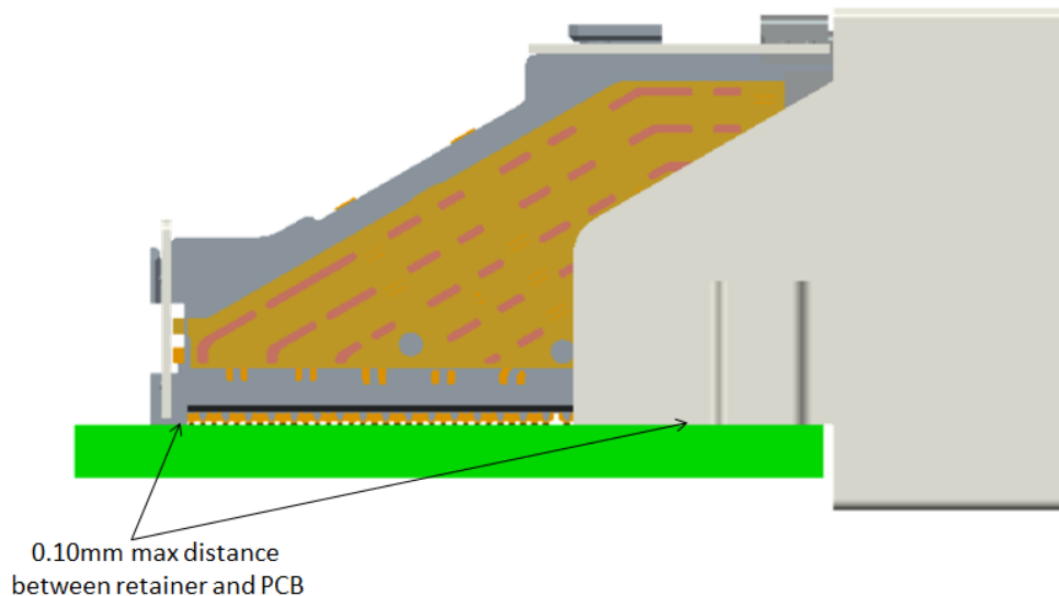
Figure 9: Proper seating depth
