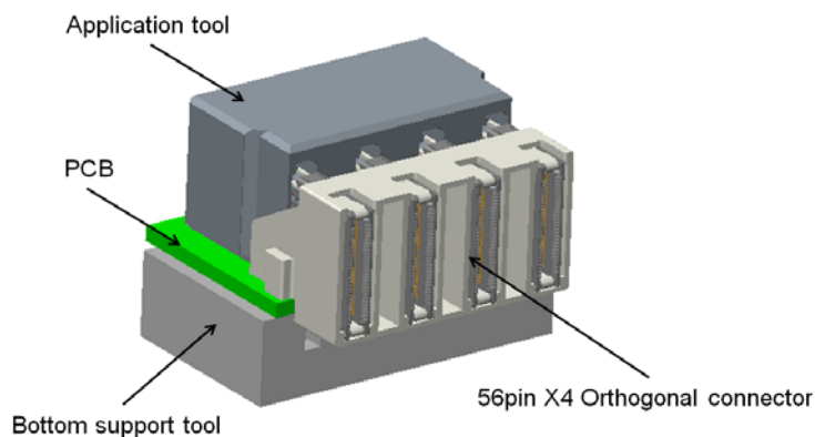
Figure 5: Orthogonal MINI Cool edge connectors x4 application tools
