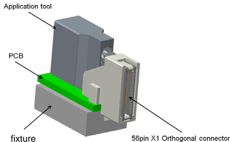
Figure 7: Orthogonal Cool edge MINI connectors 1X1 application tools
