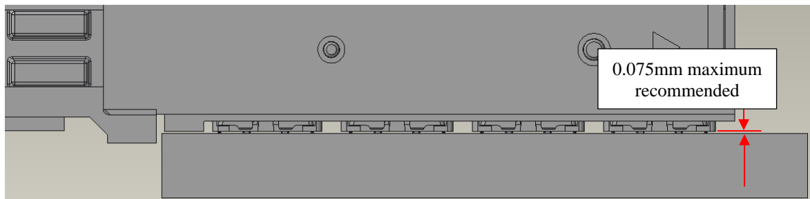
Figure 8: 0.075mm maximum height off board surface (side view)
