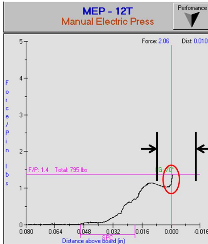
Figure A-11. Press sequence force gradient termination.
