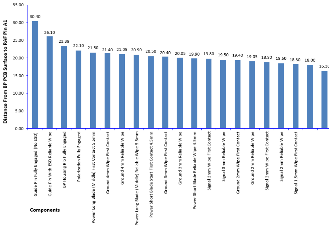
XCede HD2 3 Pair Mating Sequence
